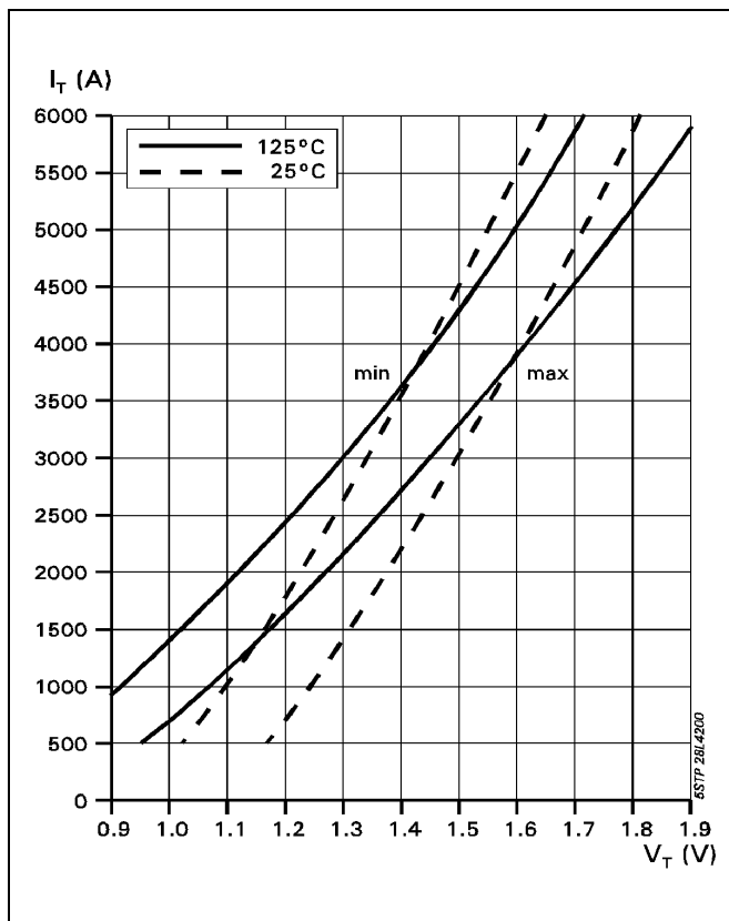
Fig. 3 On-state characteristics.
