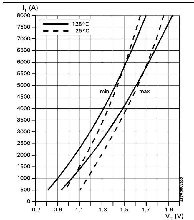
Fig. 3 On-state characteristics.
